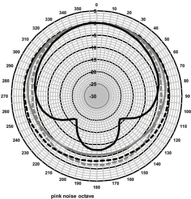
Polar diagrams (measured with pink noise)
