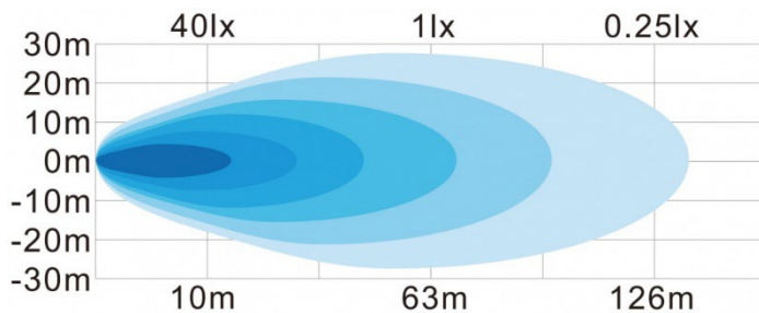
Flood Beam
