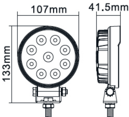
Flood Beam
